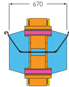
PZ27 - PILES SINGLY
